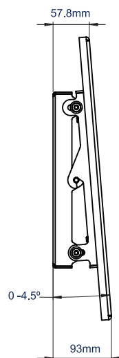
SIDE VIEW WITH -4.5° TILT
